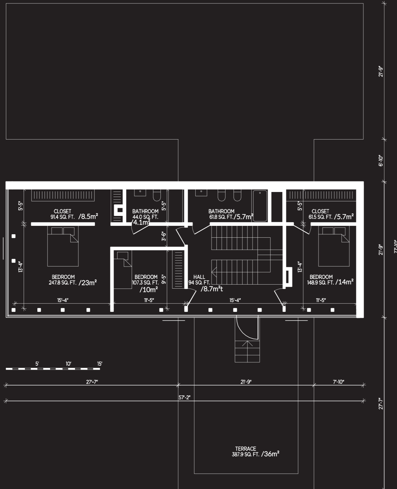
UPPER FLOOR PLAN USABLE FLOOR AREA 856.7 SQ. FT. / 80m 2
